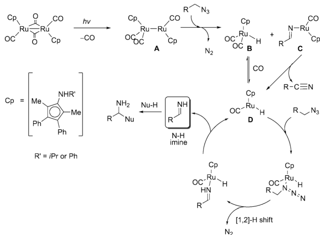
Scheme 2. Proposed mechanism for the imine formation.
